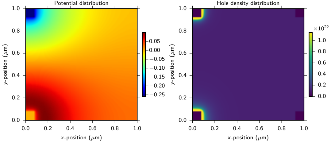
Abbildung 2.14: Calculated potential and hole-density distributions in the lateral van der Pauw structure. The potential map is obtained by iteratively solving Poisson’s equation on the two-dimensional grid with fixed contact potentials and insulating outer boundaries. The hole-density map is then calculated from the Boltzmann approximation and shows hole accumulation near the current-carrying contacts.
