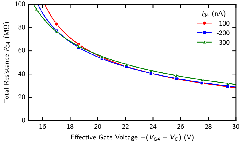
Abbildung 4.8: Total resistance R_{34} = |V_{34}/I_{34}| versus effective gate voltage V_{\text{eff}} = -(V_{G4} - V_C) for three imposed currents. The resistance decreases with increasing V_{\text{eff}} , and the three current series nearly overlap, with a small upward shift for the -300 nA series at larger V_{\text{eff}} .
