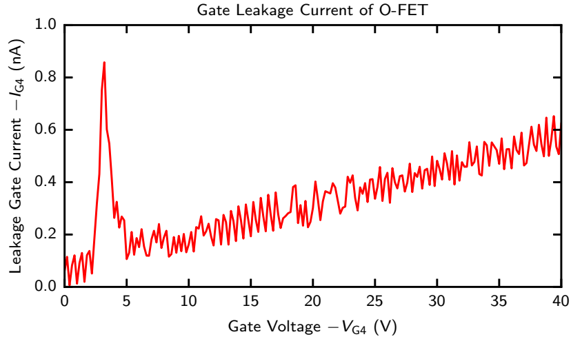
Abbildung 4.2: Gate-insulator leakage current of the gated thin-film structure, measured as -I_{G4} while sweeping the gate voltage -V_{G4} . The leakage current remains in the nanoampere range over the full voltage sweep, well below the 1\text{ }\mu\text{A} limit. The isolated peak at low gate voltage is interpreted as a transient caused by a small dust particle, which is subsequently swept out by the applied electric field.
