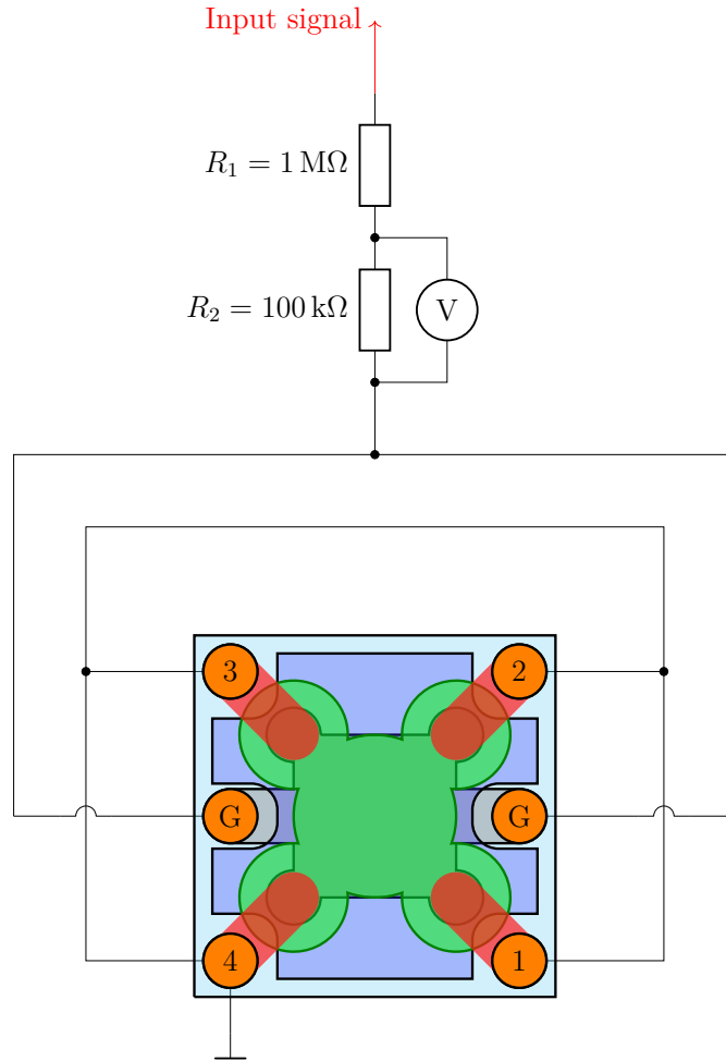
Abbildung 4.9: Circuit used for the deep-level transient spectroscopy (DLTS)-type measurements on the gated thin-film structure. The external excitation is applied through the resistive divider formed by R_1 = 1 \text{ M}\Omega and R_2 = 100 \text{ k}\Omega . The voltage across R_2 is monitored so that the transient response of the device can be followed after each bias perturbation.
