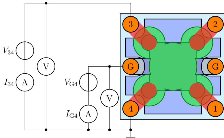
Abbildung 4.1: Circuit used for the current-voltage characterization of the gated thin-film structure. The source-drain branch measures V_{34} and I_{34} between contacts 3 and 4, while the gate branch applies V_{G4} and monitors the gate leakage current I_{G4} . Adapted from the figures in the internal laboratory archive.
