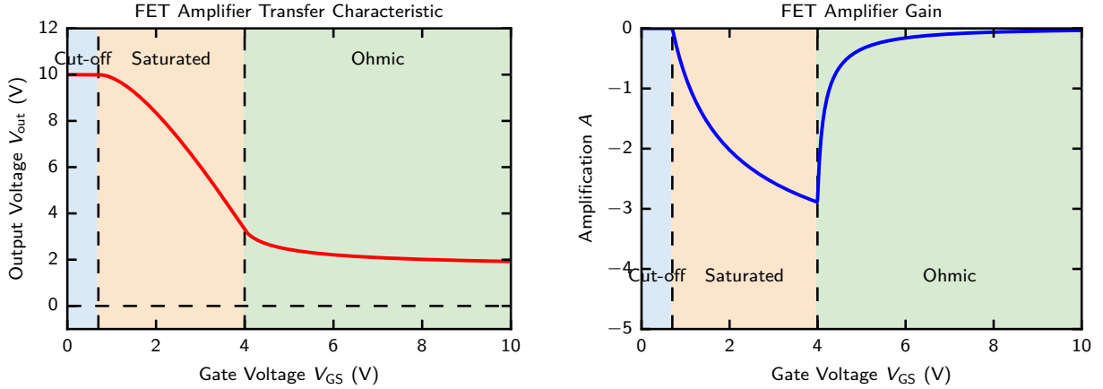
Abbildung 2.12: FET amplifier transfer characteristic and small-signal gain. The left panel shows the static output voltage as a function of gate bias. The local slope of this curve determines the voltage gain shown on the right. The gain is negative in the inverting common-source configuration and is largest in magnitude within the transition region between cut-off and strongly ohmic operation.
