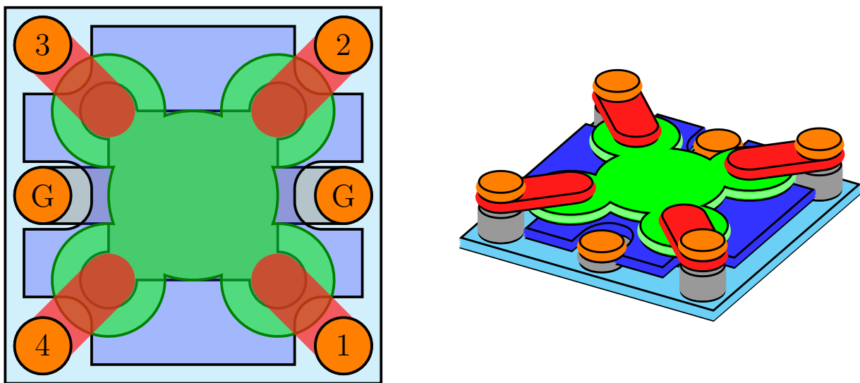
Abbildung 3.2: Schematic representation of the assembled thin film structure. The left panel shows the top-view contact layout, while the right panel shows the corresponding 3D layer structure.
