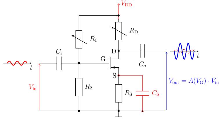
Abbildung 2.11: Common-source FET amplifier with a resistive drain load, gate-bias network, source stabilization, and coupling capacitors. The source-bypass capacitor increases the AC gain by suppressing source degeneration over its effective frequency range. The output signal is amplified and inverted relative to the input signal.
