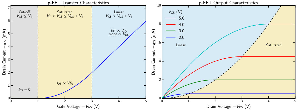
Abbildung 2.9: Idealized transfer characteristic at fixed drain bias (left) and output characteristics at several gate voltages (right). For consistency with Equation 2.34, the axes show the magnitudes of the p -channel voltages and current. In the linear regime, I_D is approximately linear in gate overdrive and drain voltage. In saturation, I_D is approximately quadratic in gate overdrive and ideally independent of drain voltage.
