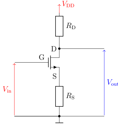
Abbildung 2.10: FET used as a voltage-controlled switch in a resistive circuit. A change of gate voltage changes the channel resistance and therefore the output voltage at the drain. The schematic uses the conventional n -channel polarity; a p -channel implementation requires reversed polarities.
