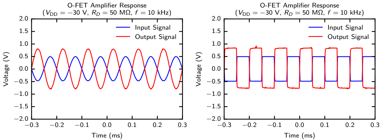
Abbildung 4.14: Dynamic response of the thin-film amplifier at V_{DD} = -30 V, R_D = 50 M \Omega , V_{G,Q} = -18 V, and f = 10 kHz. The sinusoidal measurement demonstrates inverted voltage amplification, while the square-wave measurement shows the finite rise and fall times caused by the large circuit resistance, device capacitance, and trap-related relaxation.
