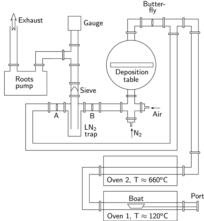
Abbildung 3.5: Schematic of the chemical vapor deposition (CVD) system used for PaN deposition. Adapted from the figures in the internal laboratory archive.
