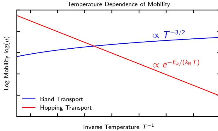
Abbildung 2.7: Schematic temperature dependence of charge transport in organic semiconductors. Thermally activated hopping typically becomes more efficient at higher temperature, whereas band-like transport can decrease with increasing temperature because molecular vibrations disturb intermolecular coupling.
