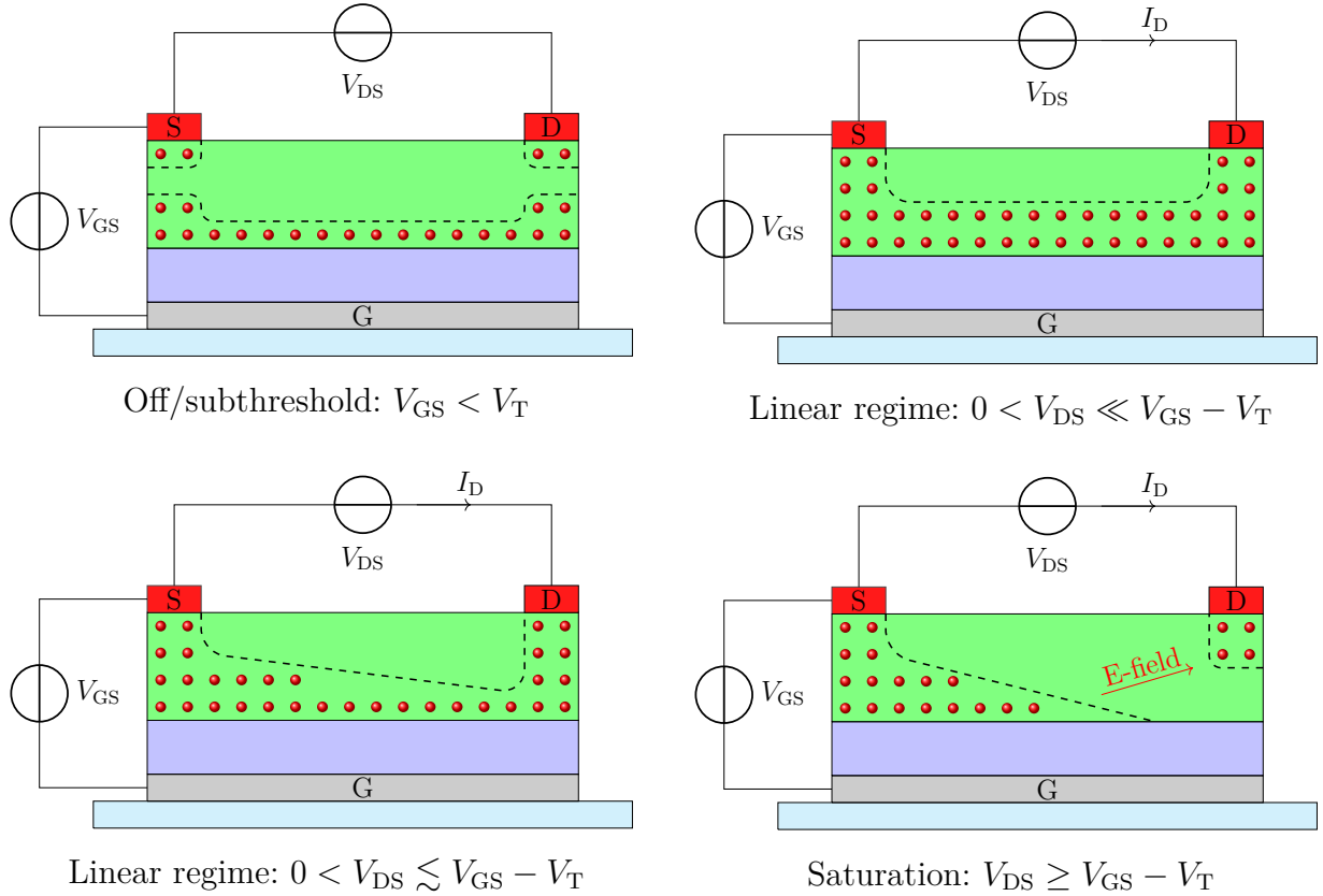
Abbildung 2.8: Schematic side views of the main operating regimes of a p -channel field-effect transistor. The voltage labels denote the positive bias magnitudes defined in Equation 2.34. Increasing gate bias forms a hole accumulation layer at the semiconductor–dielectric interface. Increasing drain bias makes the channel charge nonuniform and eventually produces pinch-off near the drain.
