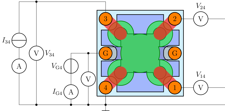
Abbildung 4.6: Gated van der Pauw measurement circuit used to extract the intrinsic sheet conductance. A constant current I_{34} is driven between contacts 3 and 4 while the voltage V_{34} is monitored. The transverse probe voltages V_{14} and V_{24} are measured with high-impedance voltmeters, and the gate branch applies V_{G4} while monitoring the leakage current I_{G4} . Adapted from the figures in the internal laboratory archive.
