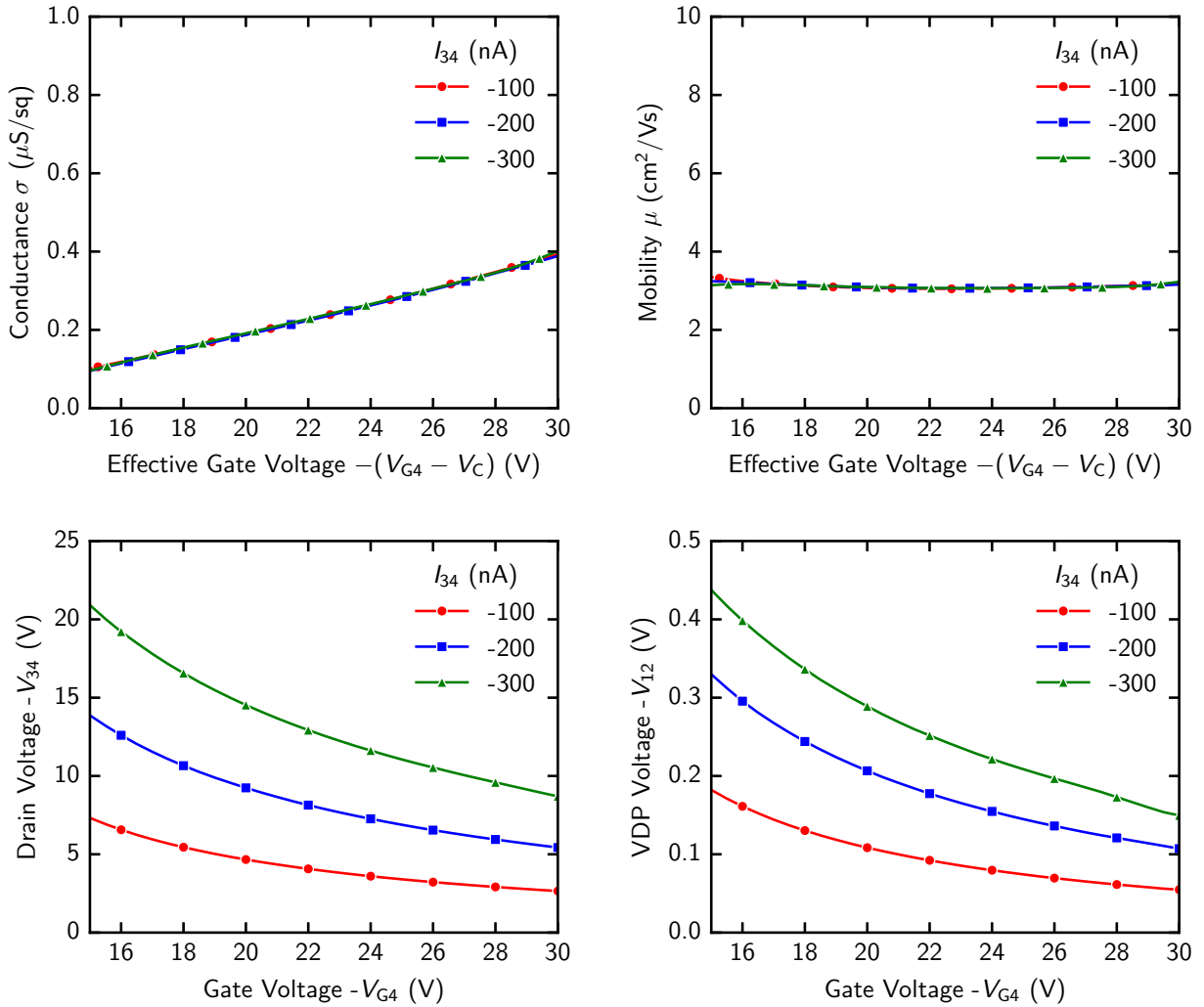
Abbildung 4.7: Gated van der Pauw extraction for I_{34} = -100 \text{ nA} , -200 \text{ nA} , and -300 \text{ nA} . The lower panels show the measured voltages, while the upper panels show the extracted sheet conductance \sigma and mobility versus effective gate voltage. The overlap of the three current series indicates linear-response behaviour and supports a current-independent mobility extraction.
