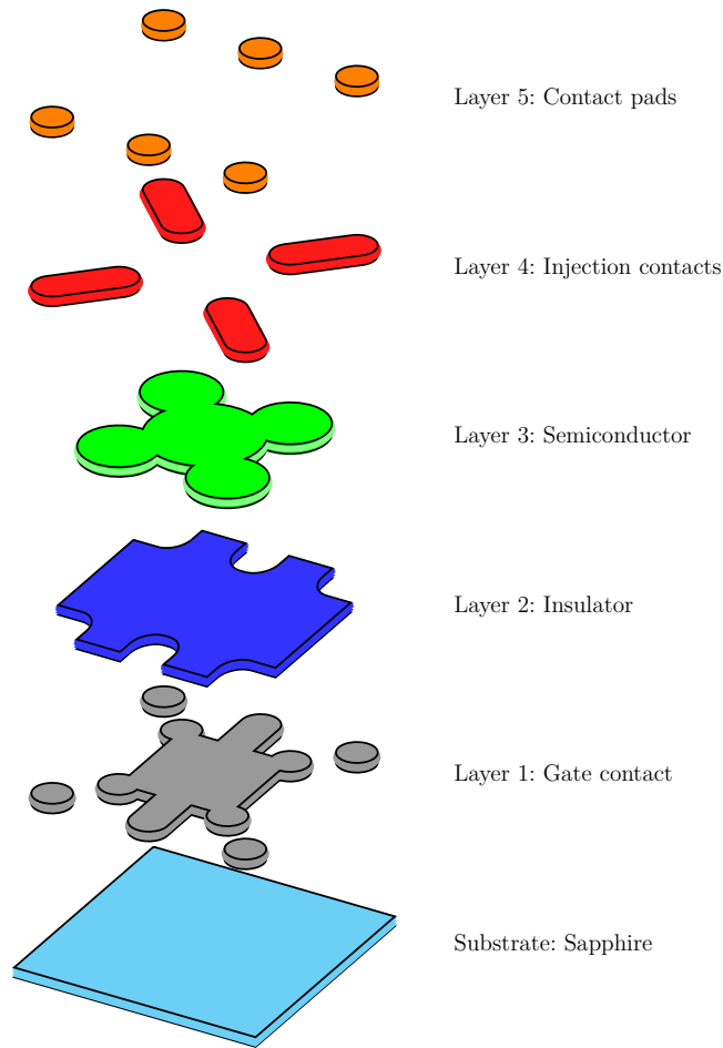
Abbildung 3.1: Device layout used for electrical characterization. The structure contains a bottom gate, a dielectric stack, a molecular semiconductor layer, four injection contacts, and larger contact pads for external wiring. Adapted from the figures in the internal laboratory archive.
