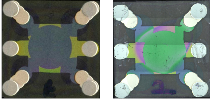
Abbildung 3.7: Fabricated devices under the microscope. Left: optically well-defined device. Right: device with visible defects. Photos from internal laboratory archive.
