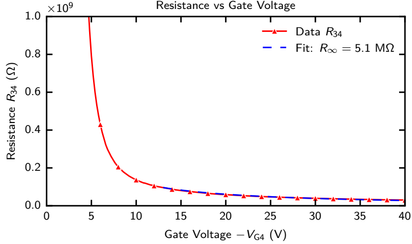
Abbildung 4.4: Drain–source resistance R_{34} = V_{34}/I_{34} extracted from the low-drain-bias linear regime as a function of gate voltage. The resistance decreases as the negative gate bias accumulates a more conductive hole channel. The fitted background resistance represents the gate-independent part of the two-terminal resistance and is attributed mainly to injection/contact resistance associated with the Schottky barrier at the metal–organic semiconductor interface.
