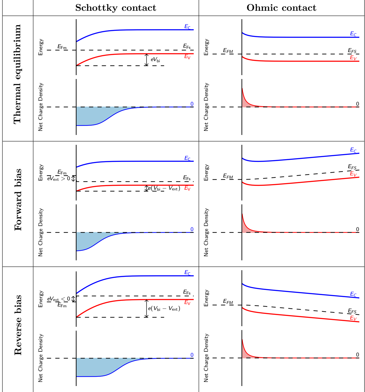
Abbildung 2.4: Band diagrams and corresponding net charge-density profiles for metal–semiconductor contacts under equilibrium, forward-bias, and reverse-bias conditions.
