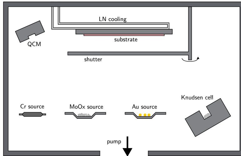
Abbildung 3.3: Schematic of the physical vapor deposition (PVD) system. Figure from Ref. [22].
