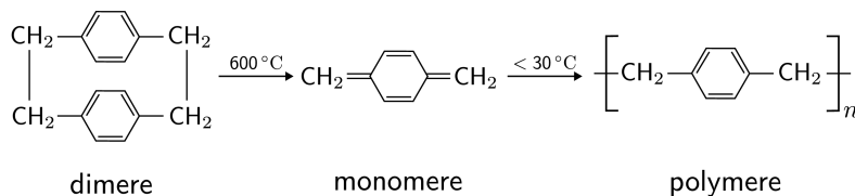
Abbildung 3.4: Schematic of the chemical synthesis of parylene-N (PaN). Figure from Ref. [22].
