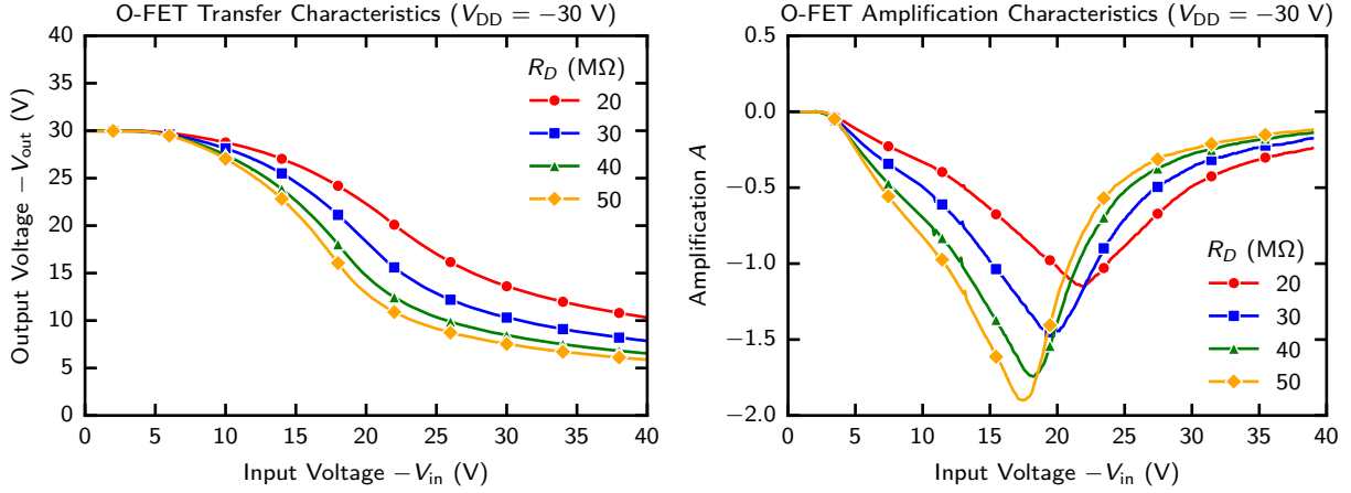
Abbildung 4.13: Transfer curve and amplification characteristic at V_{DD} = -30 V for different drain-load resistances R_D . The transfer plot identifies the input-voltage range where the output voltage changes most strongly, while the amplification plot shows the corresponding small-signal voltage gain. Larger R_D values increase the maximum gain but also narrow the useful operating range.
