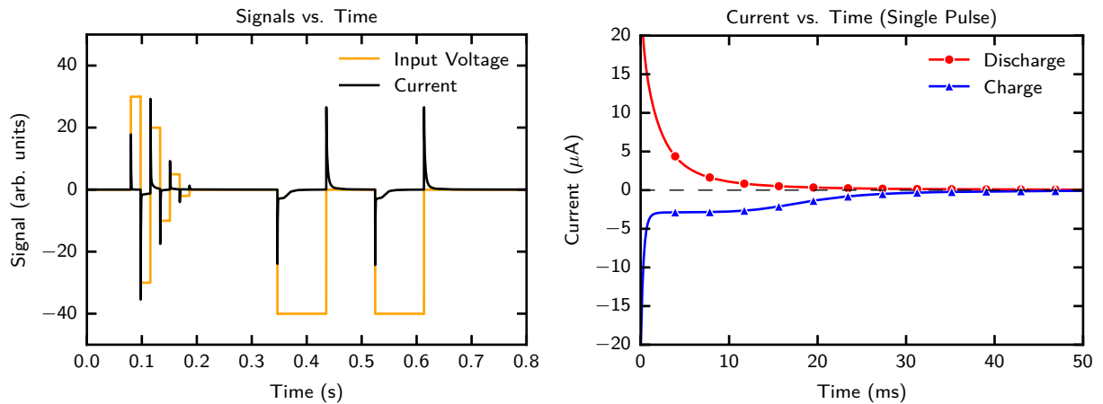
Abbildung 4.10: DLTS excitation waveform and representative single-pulse transient response. The left panel shows the applied voltage pulses together with the corresponding current response. The right panel compares the charge and discharge transients after one pulse, showing a fast initial response followed by a slower relaxation towards the baseline.
