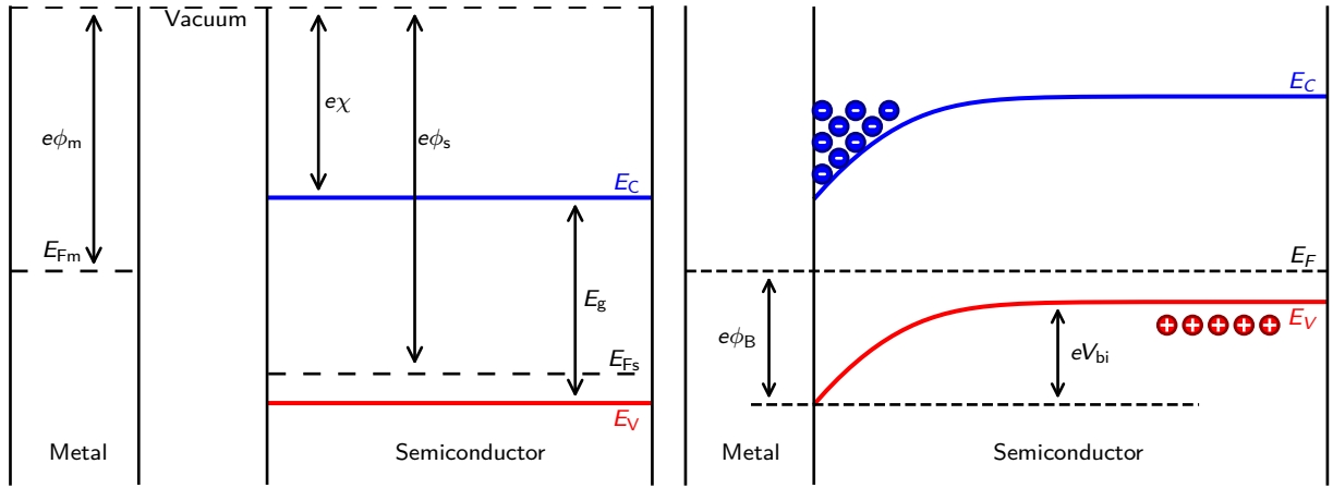
Abbildung 2.3: Schottky barrier formation at a metal– p -type semiconductor contact. Band alignment of a metal and a p -type semiconductor before (left) and after contact (right). Fermi-level alignment causes band bending in the semiconductor and can form a Schottky barrier for hole transport.
