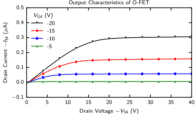
Abbildung 4.5: Output characteristic of the organic FET, measured as drain current -I_{34} as a function of drain voltage -V_{34} for different fixed gate voltages V_{G4} .
