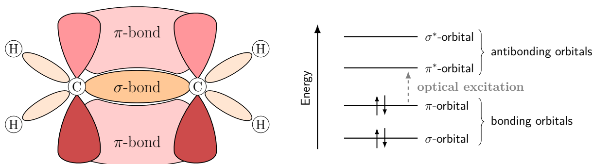
Abbildung 2.6: Sigma and pi bonding in ethene as the simplest conjugated pi-electron system. The left panel illustrates the spatial overlap of the \sigma and \pi bonds, while the right panel shows the corresponding bonding and antibonding orbital levels. The lowest optical excitation occurs from the bonding \pi orbital to the antibonding \pi^* orbital. Adapted from Ref. [22] and [13].
